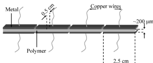
Fig. 4 Schematic Ionic Polymeric Metal Composite worm presented in Kim et al. [2].
