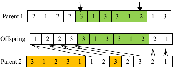
Fig. 3 Illustration of the enhance order crossover
