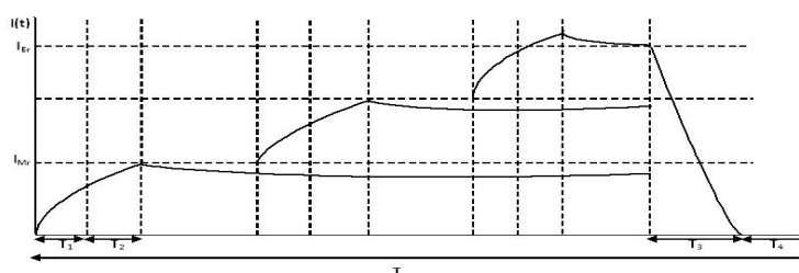
Fig. 3 Inventory level of imperfect items in 3 production setups and 1 rework setup.
