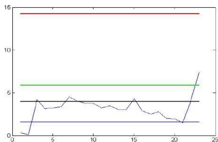
Fig. 2 Trace plot of the Variable parameter Generalized Likelihood Ratio statistic.
